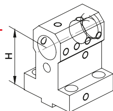
W1417 D32 - H=55 mm (Ø32 mm) Z2417 D32 - H=70 mm (Ø32 mm) Z7417 D32 - H=80 mm (Ø32 mm)
