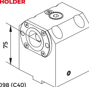
POLYGONAL TOOL HOLDER
