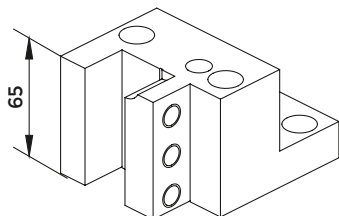
FACE AND O.D. CUTTING HOLDER
